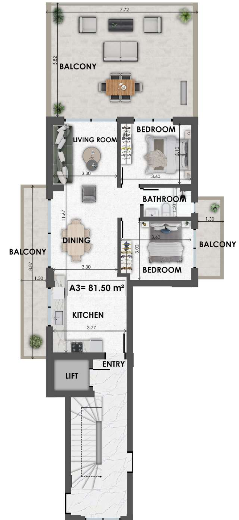
A3 - 2 nd Floor Plan
