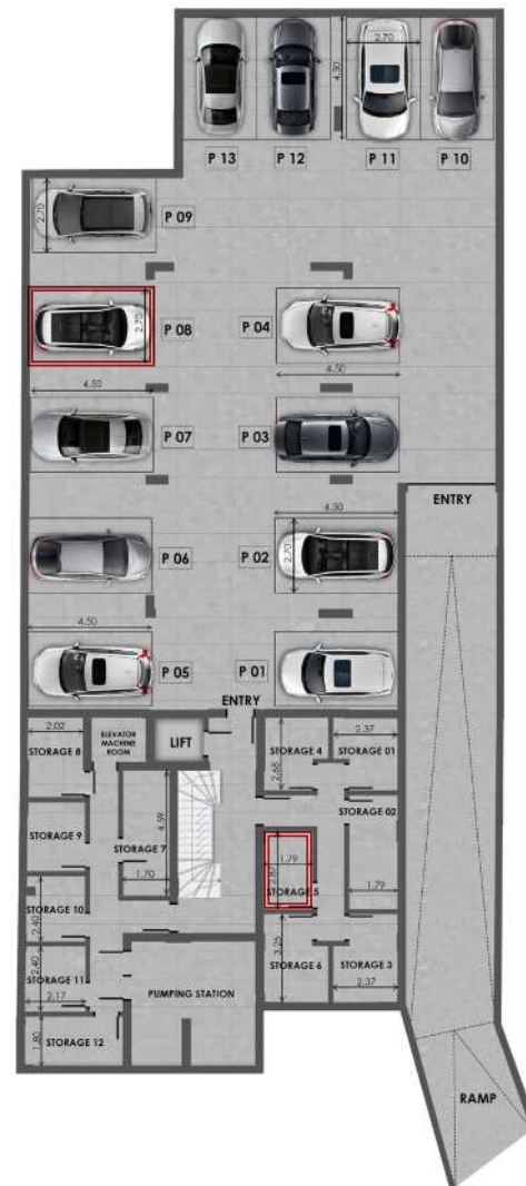
A3 - UNDERGROUND Parking / Storage
